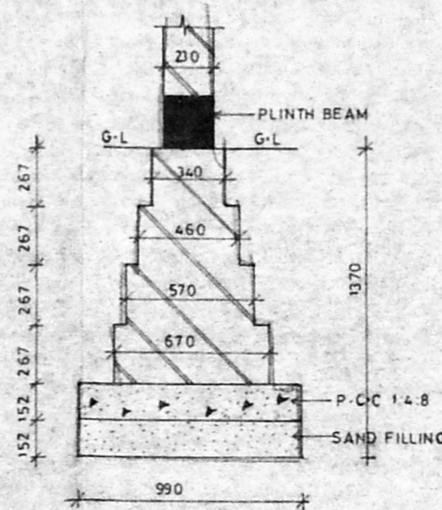
Detail of Brickwall Foundation
